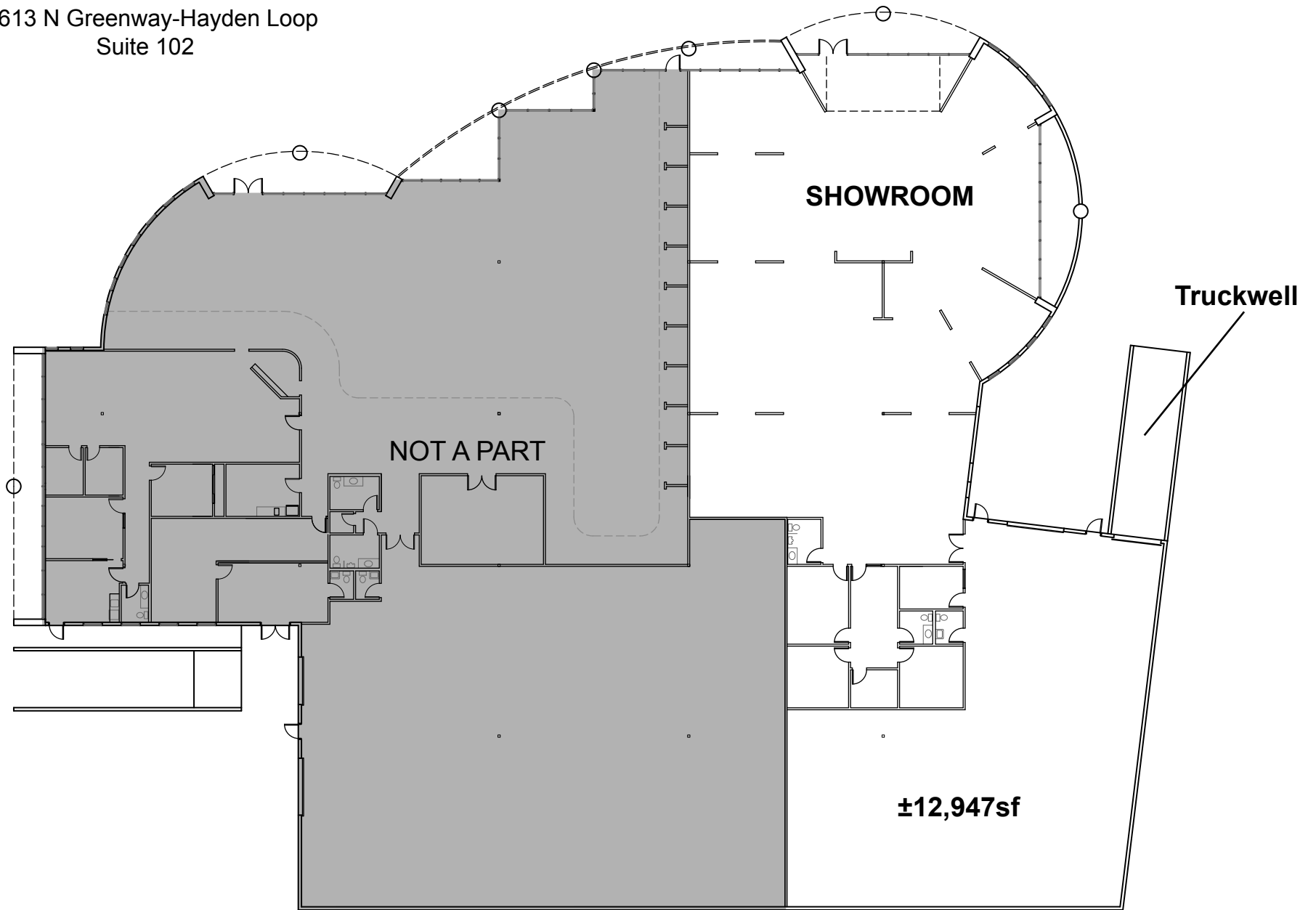
FLOOR PLAN
